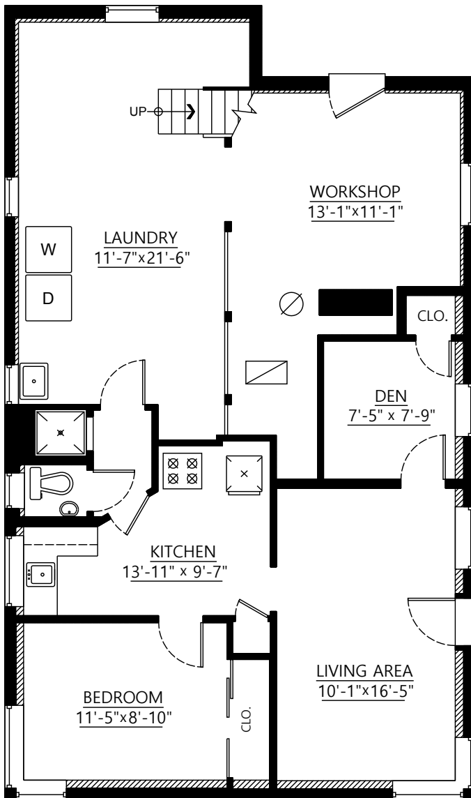
Lower Floor Plan Floor Area: 1,133 sq.ft.
