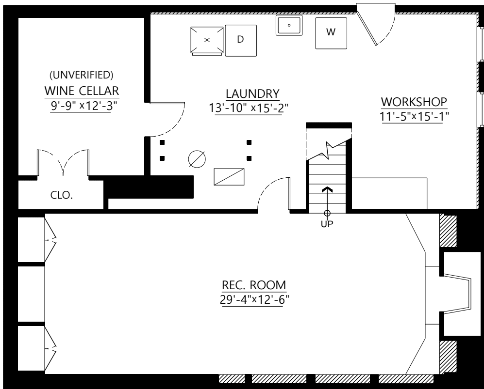
Lower Floor Plan Floor Area: 1,102 sq.ft.
