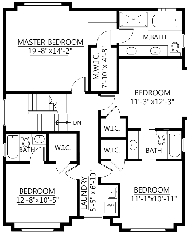
Upper Floor Plan Floor Area: 1,228 sq.ft.
