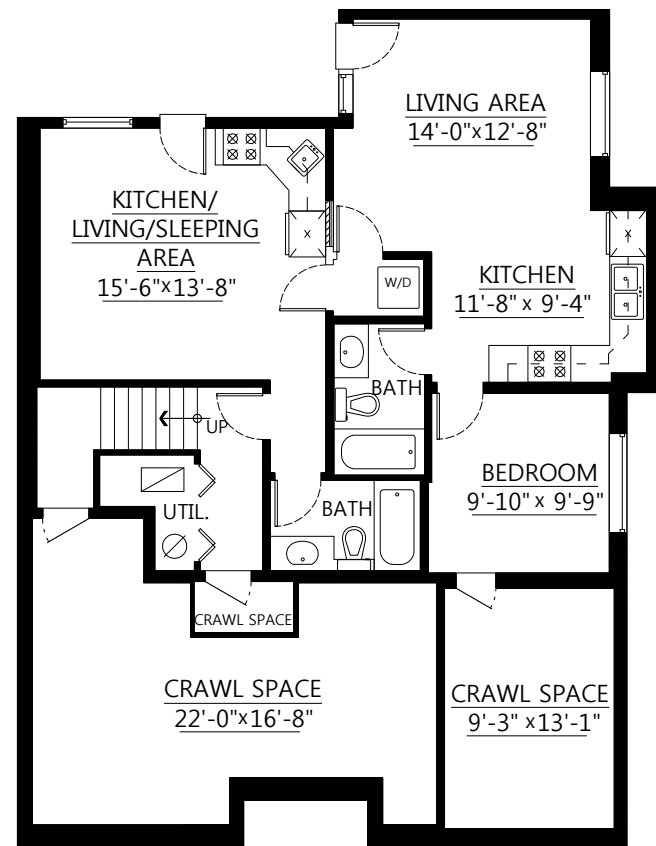
Lower Floor Plan Floor Area: 923 sq.ft.
