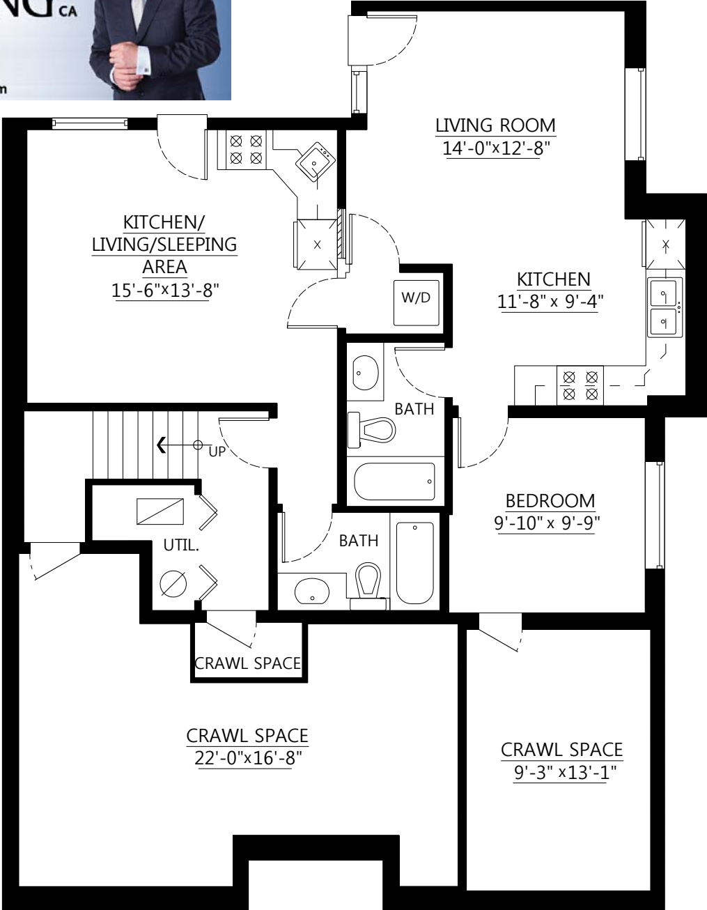
Lower Floor Plan Floor Area: 923 sq.ft.
