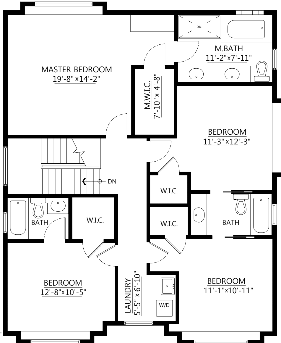
Upper Floor Plan Floor Area: 1,228 sq.ft.
