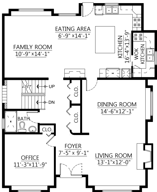
Main Floor Plan Floor Area: 1,350 sq.ft.
