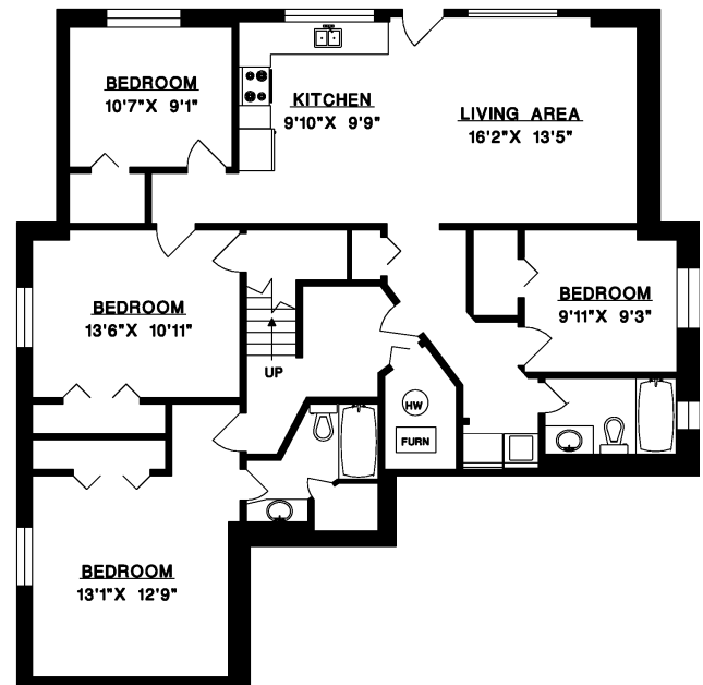
LOWER FLOOR
