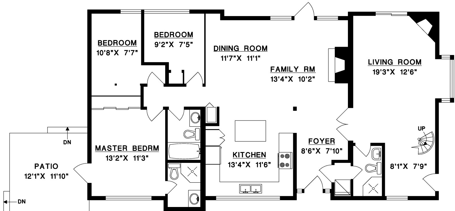
MAIN FLOOR
