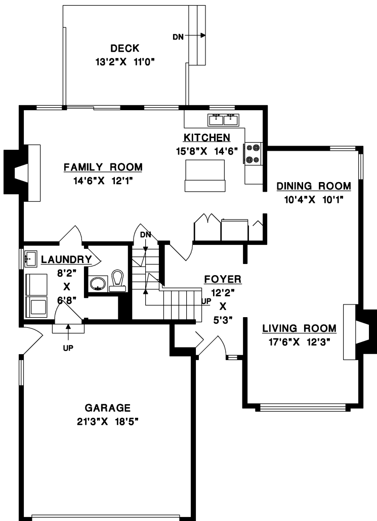
MAIN FLOOR
