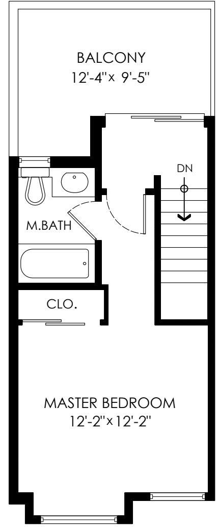
Top Floor Plan Floor Area: 320 sq.ft. Ceiling Height: 8'
