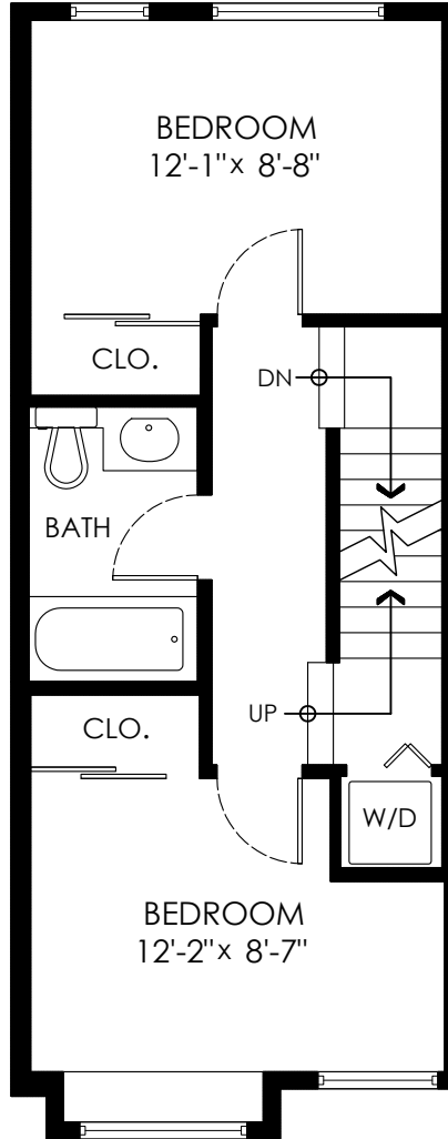
Upper Floor Plan Floor Area: 430 sq.ft. Ceiling Height: 7'-11"
