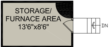
STORAGE AREA
