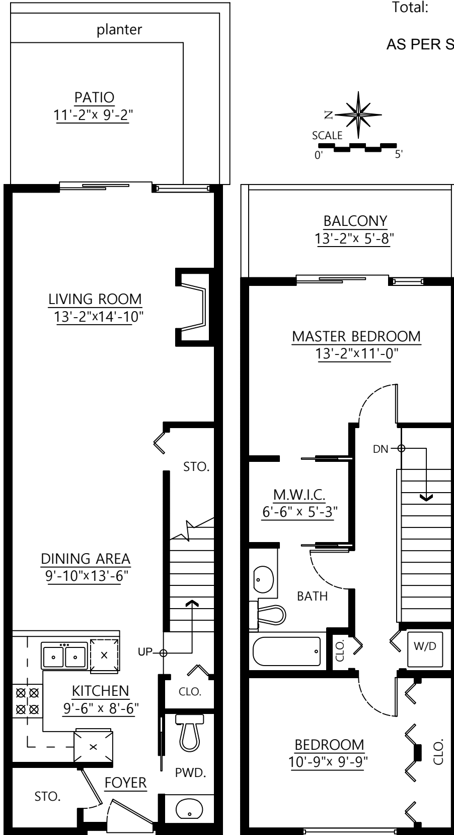
Main Floor Plan Floor Area: 592 sq.ft.
