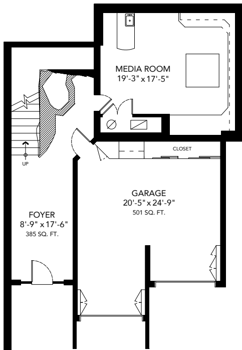
LOWER FLOOR PLAN Ceiling Height: 8'-0"
