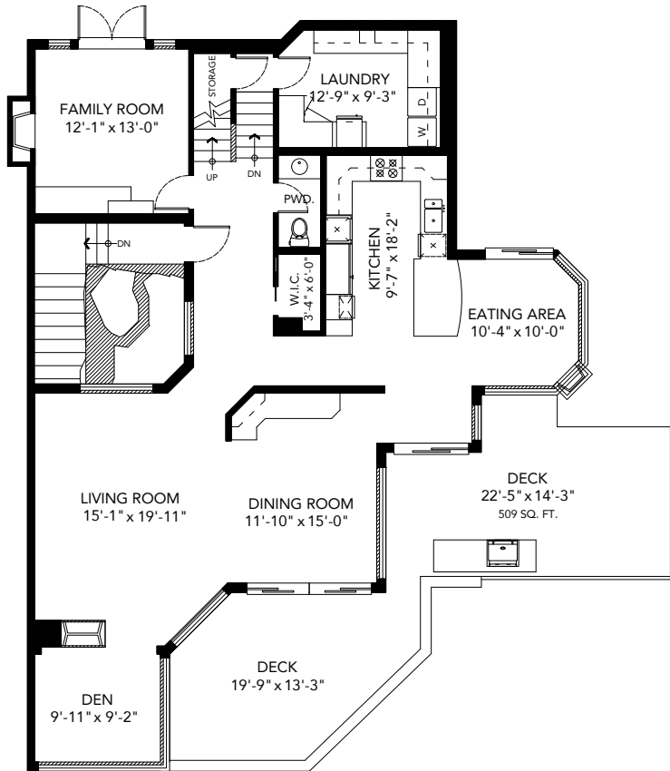
MAIN FLOOR PLAN Ceiling Height: 8'-0"
