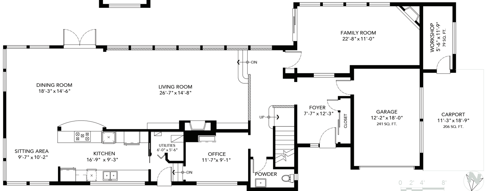
MAIN FLOOR PLAN Ceiling Height: 9'-9"
