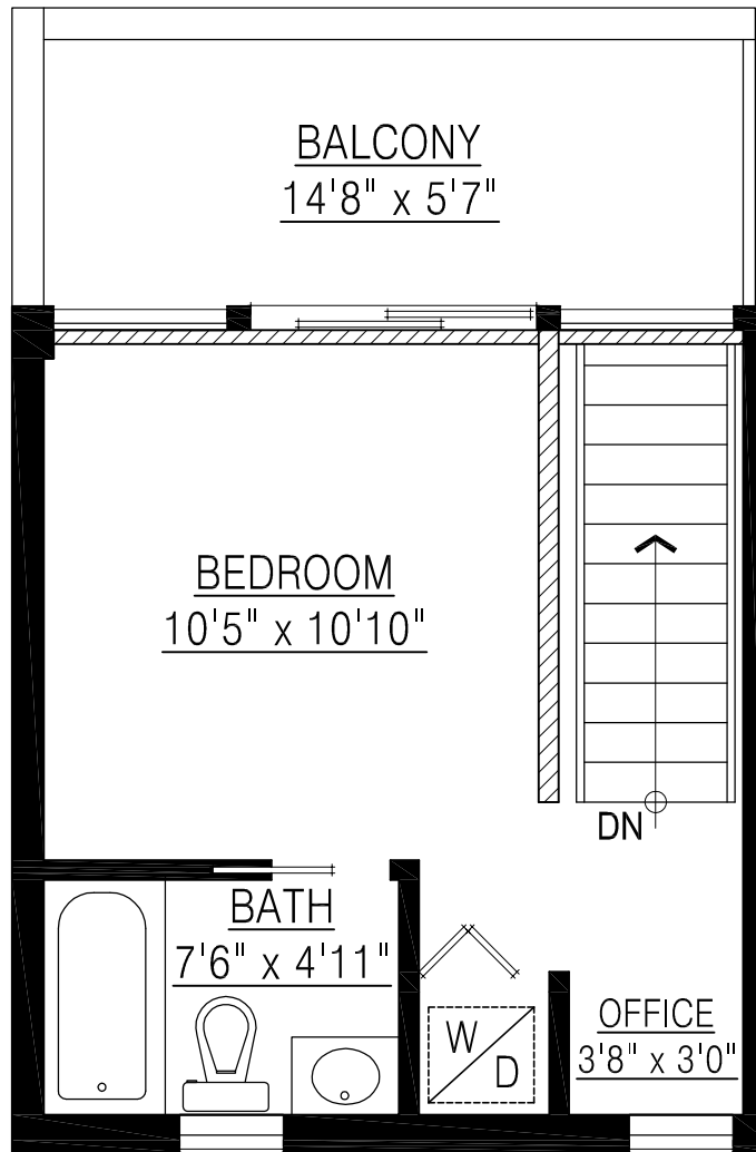
UPPER FLOOR PLAN FLOOR AREA: 273 sq.ft.
