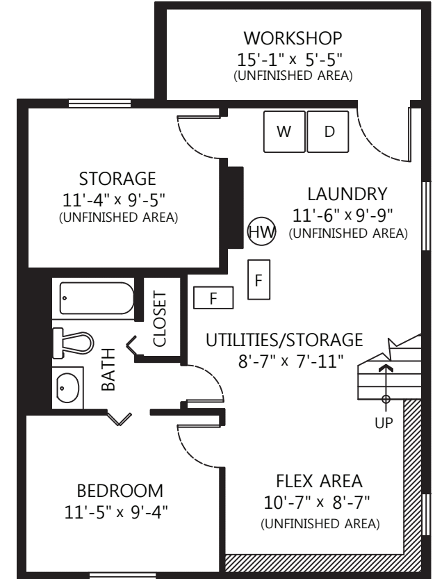
LOWER FLOOR PLAN Floor Area: 781 sq.ft.
