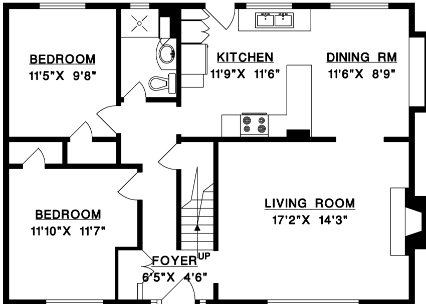
MAIN FLOOR
