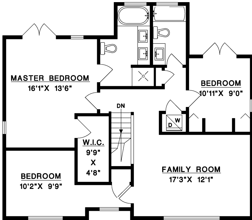
UPPER FLOOR
