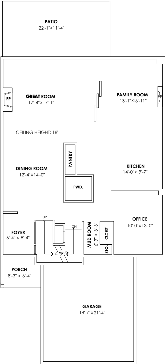
Main Floor Plan Floor Area: 1394 sq.ft. Ceiling Height: 9'
