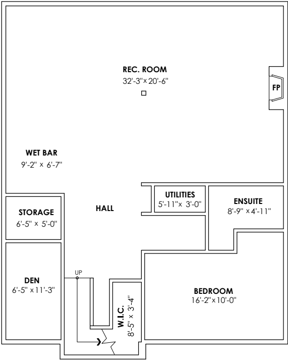
Lower Floor Plan Floor Area: 1339 sq.ft. Ceiling Height: 9'
