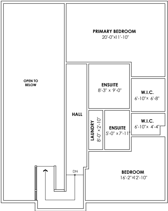
Upper Floor Plan Floor Area: 907 sq.ft. Ceiling Height: 8'
