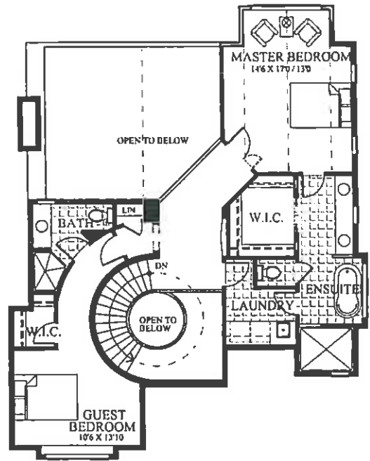
UPPER FLOOR PLAN 1,039 S.F.
