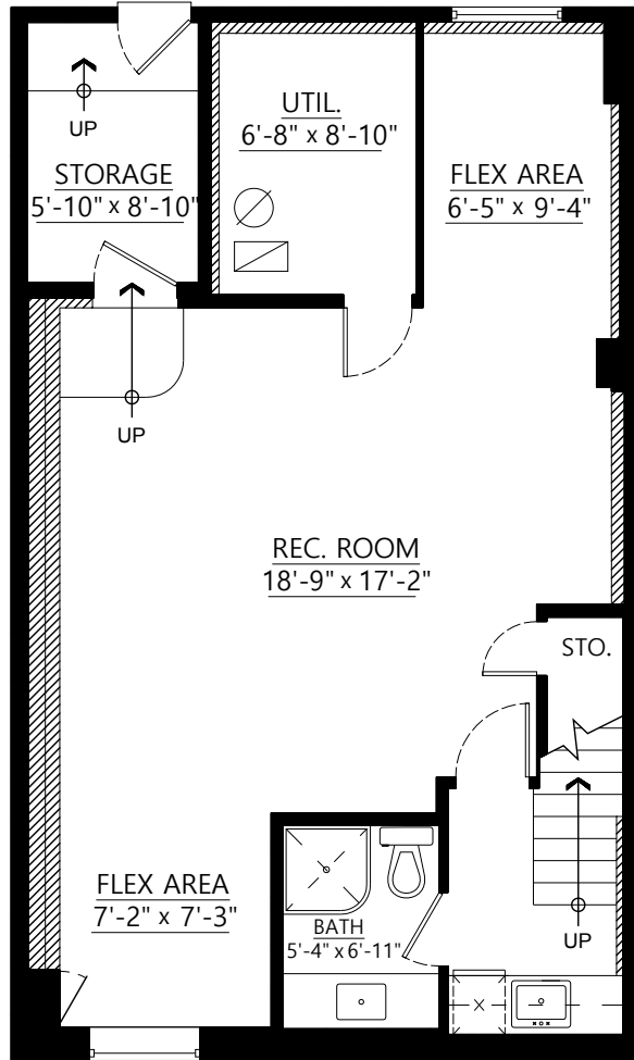
Lower Floor Plan Floor Area: 765 sq.ft.
