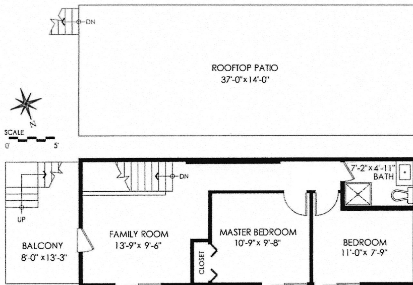
Upper Floor Plan Floor Area: 518 sq.ft. Ceiling Height: 8'-1"
