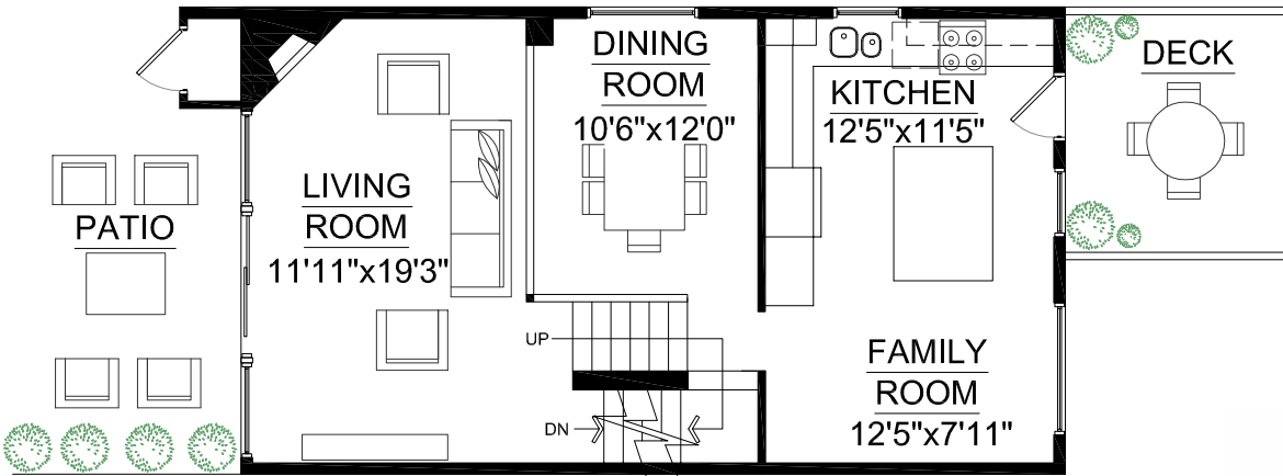
MAIN FLOOR
