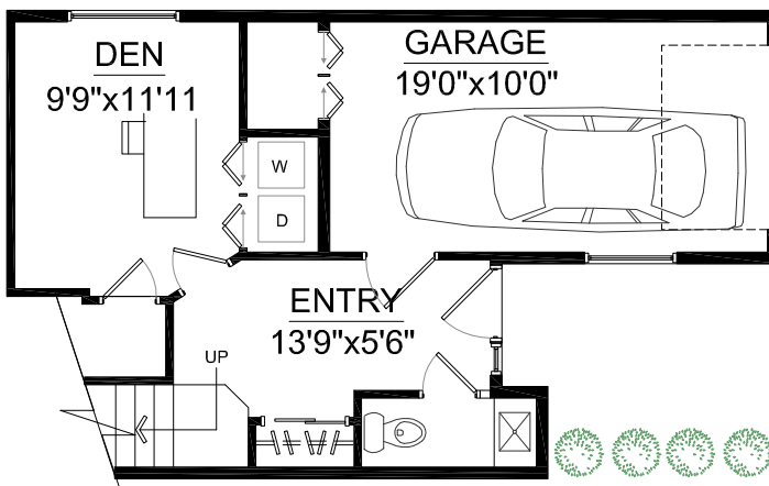
LOWER FLOOR
