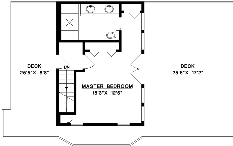
UPPER FLOOR
