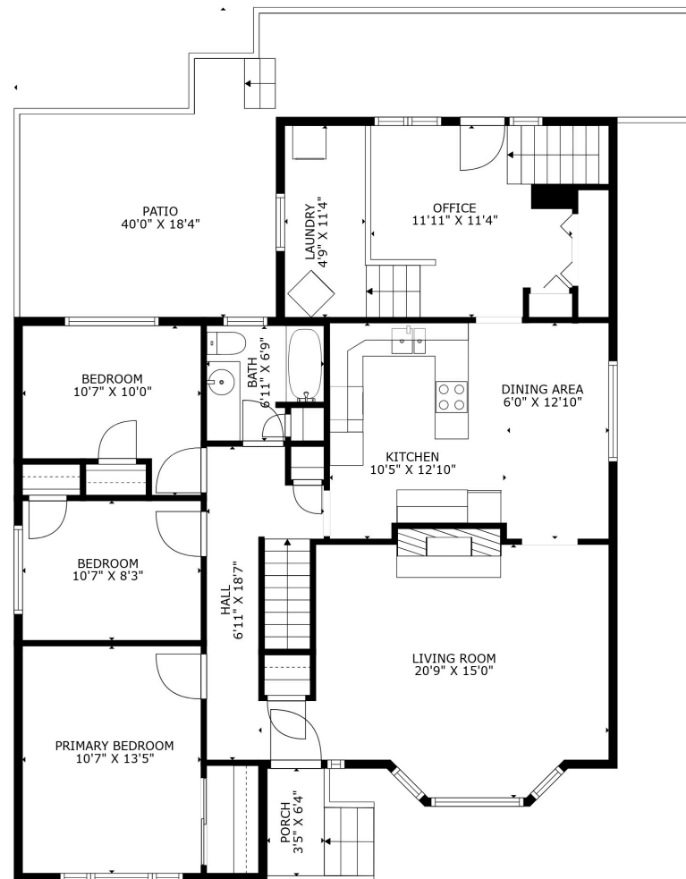
FLOOR 2
