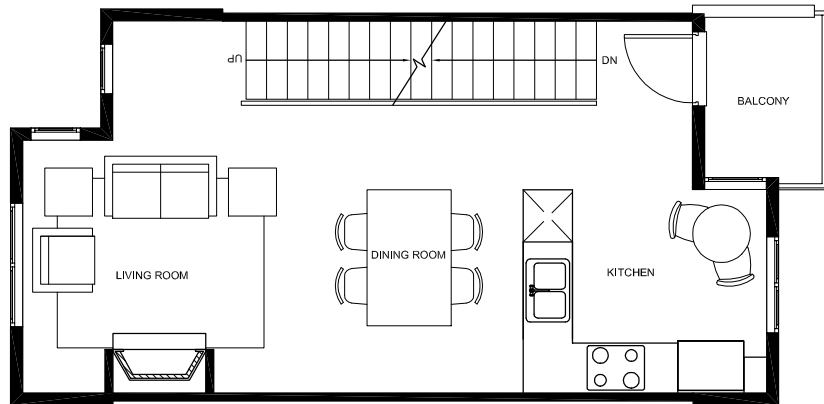
TYPE: TH-2B MAIN FLOOR PLAN
