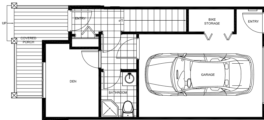
TYPE: TH-2B GROUND FLOOR PLAN
