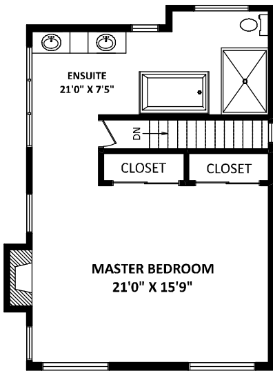
UPPER FLOOR: 694 SQ.FT.
