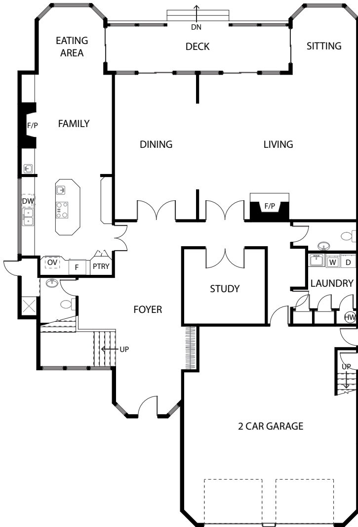
Main Floor
