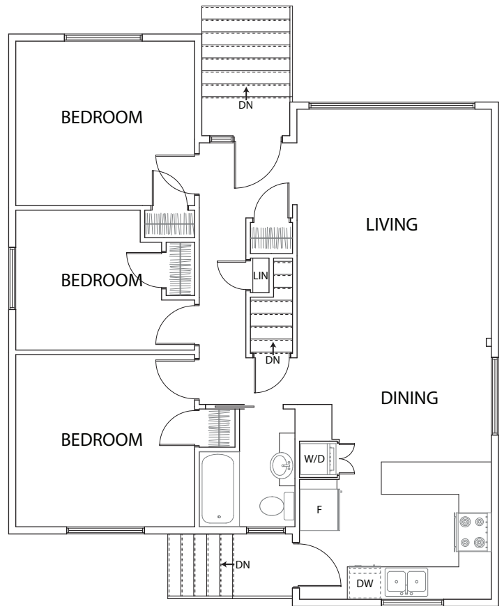
Main Floor
