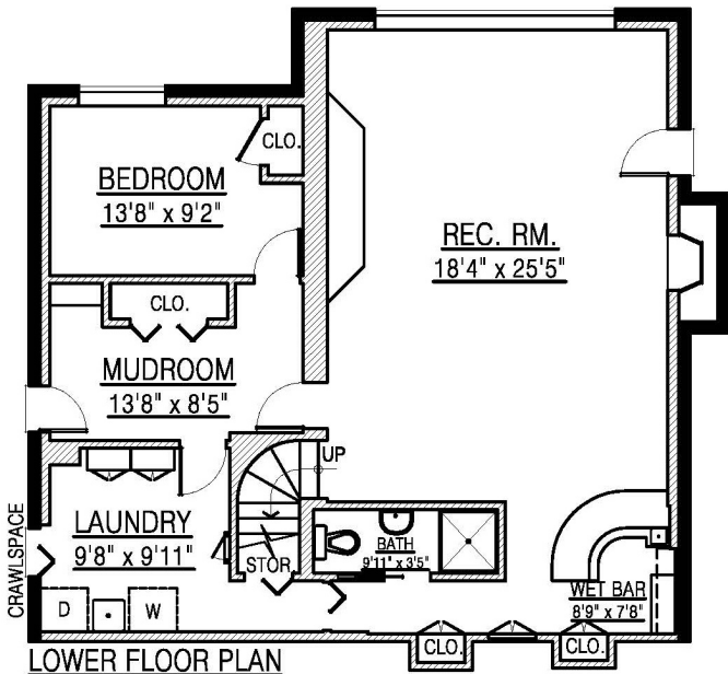
LOWER FLOOR PLAN FLOOR AREA: 1,155 sq. ft.
