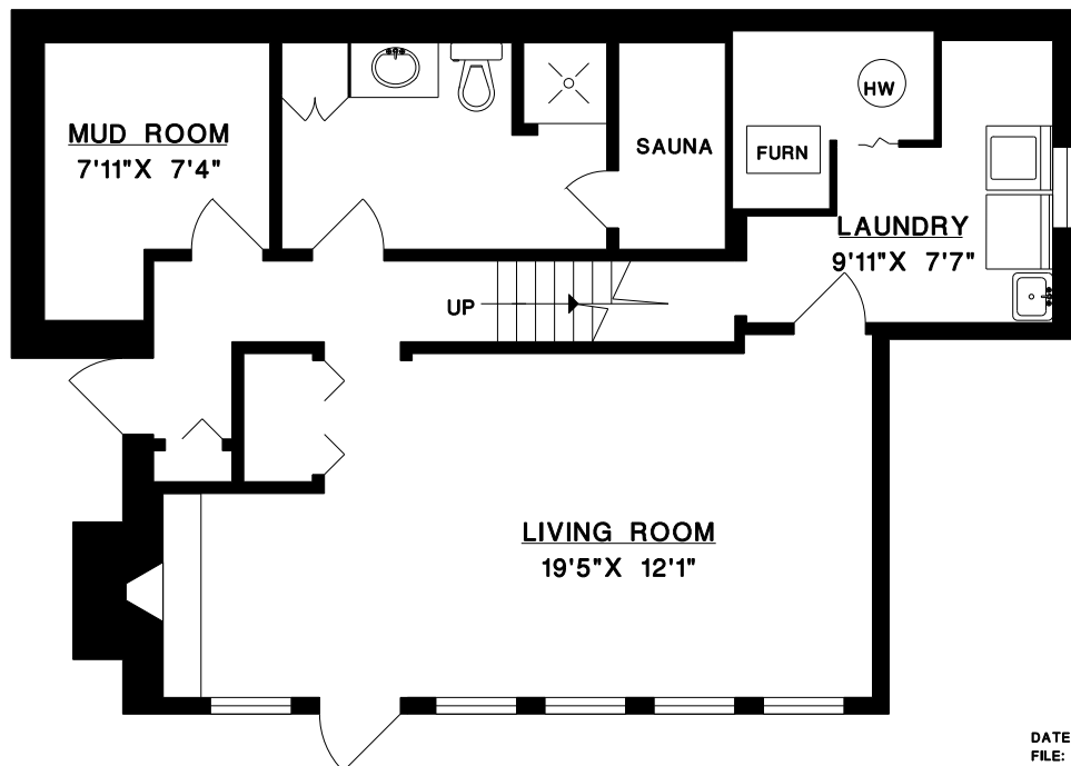
LOWER FLOOR
