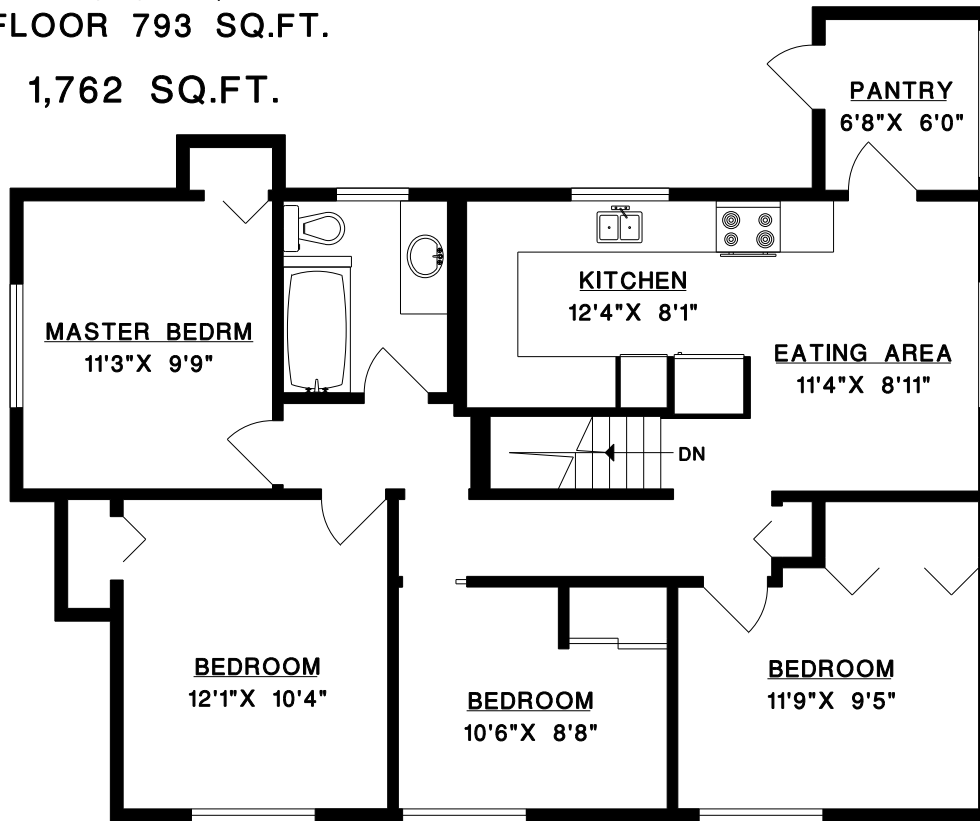
MAIN FLOOR
