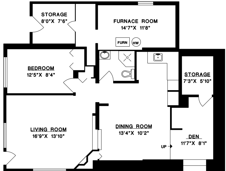
LOWER FLOOR
