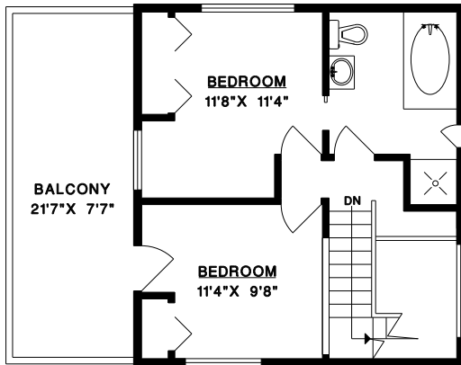
UPPER FLOOR
