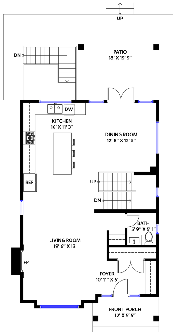
MAIN FLOOR 934 SQ.FT.
