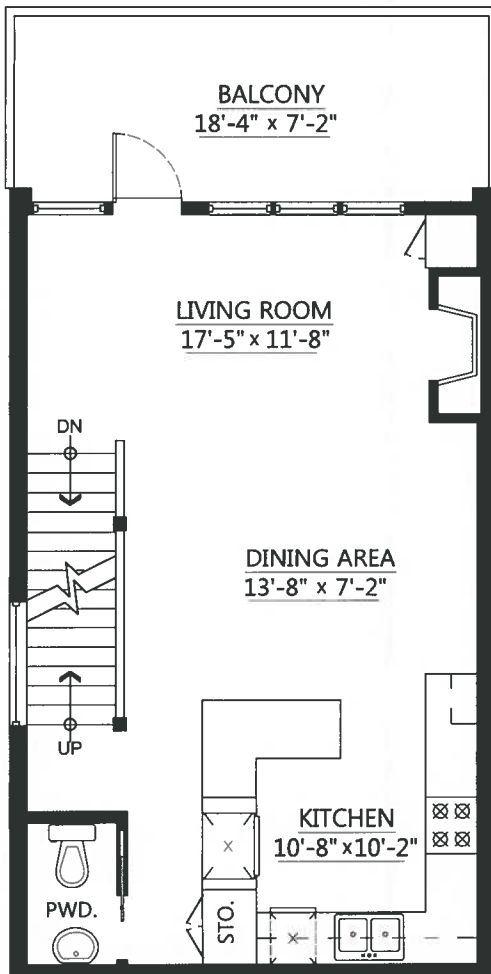
Main Floor Plan Floor Area: 562 sq.ft.
