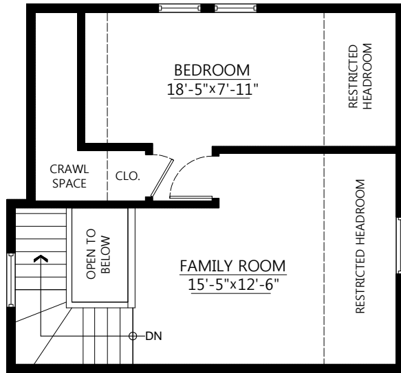
Top Floor Plan Floor Area: 320 sq.ft.
