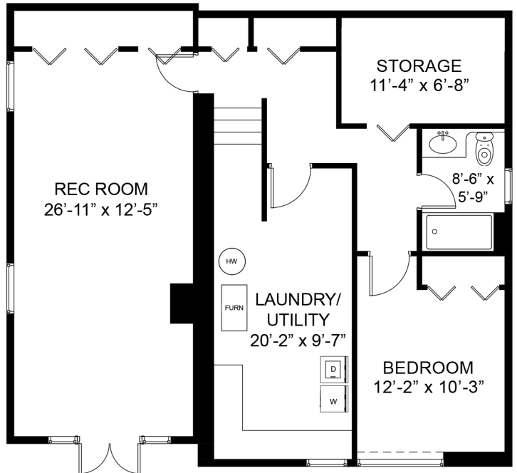
BASEMENT 1102 SQ.FT.
