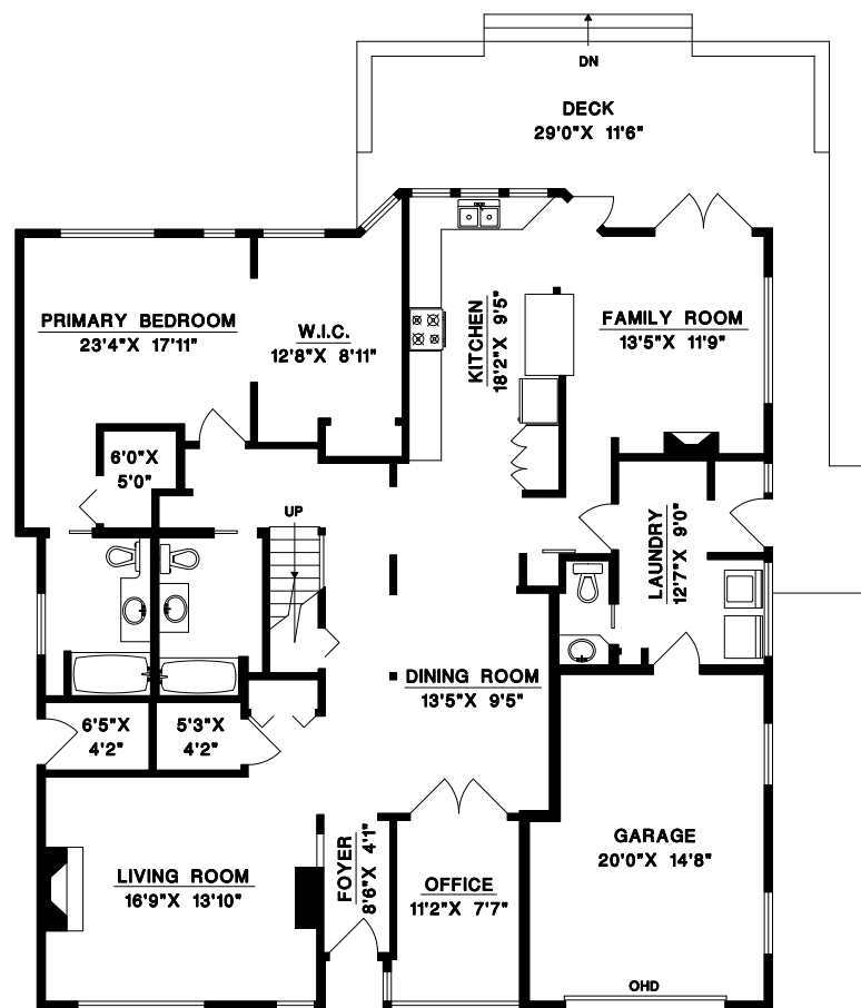
MAIN FLOOR
