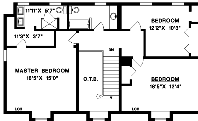
UPPER FLOOR
