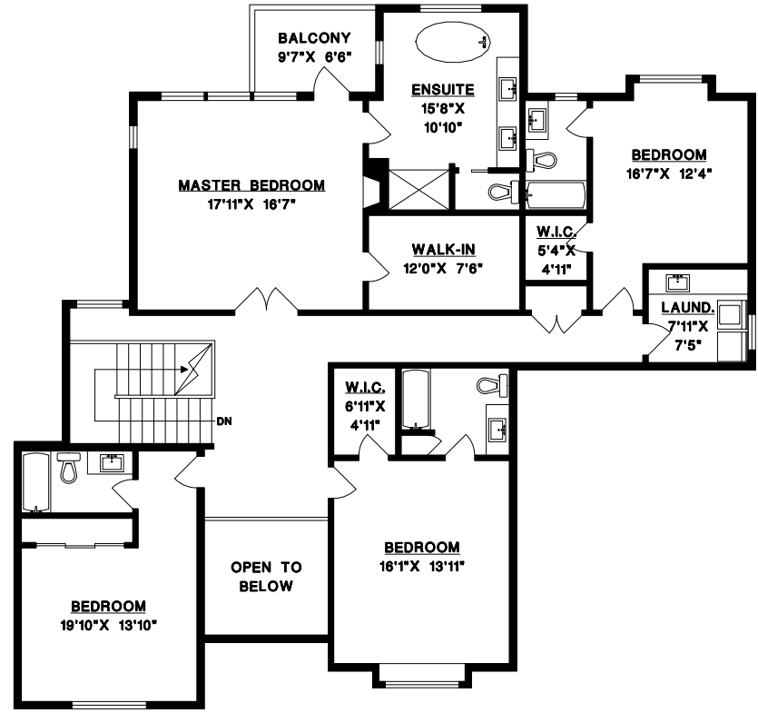
UPPER FLOOR
