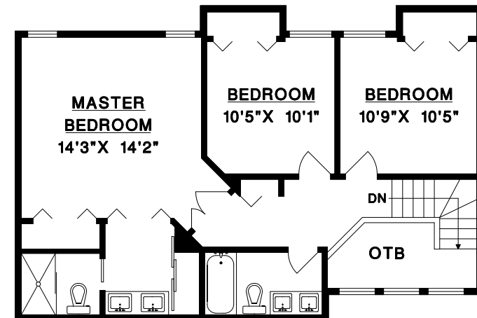
UPPER FLOOR
