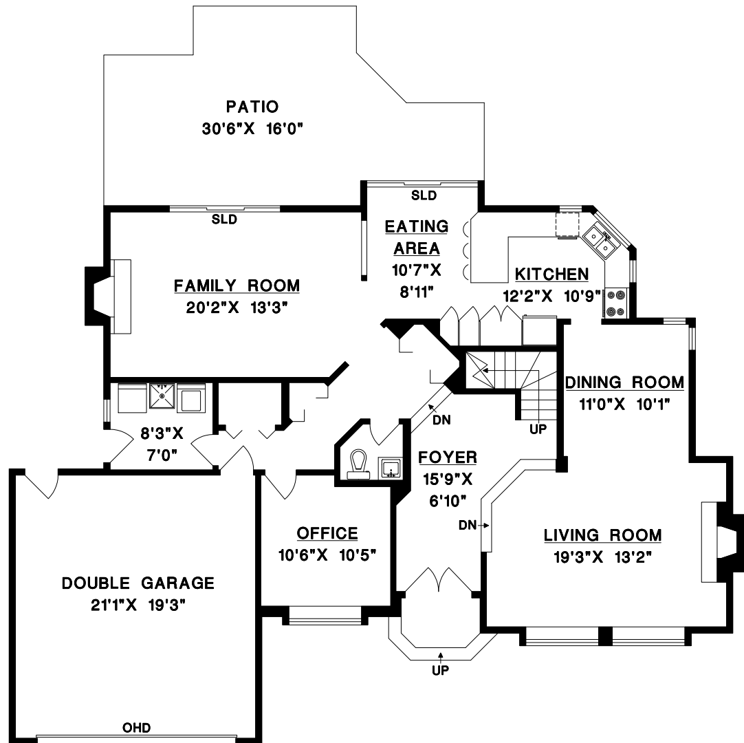
MAIN FLOOR
