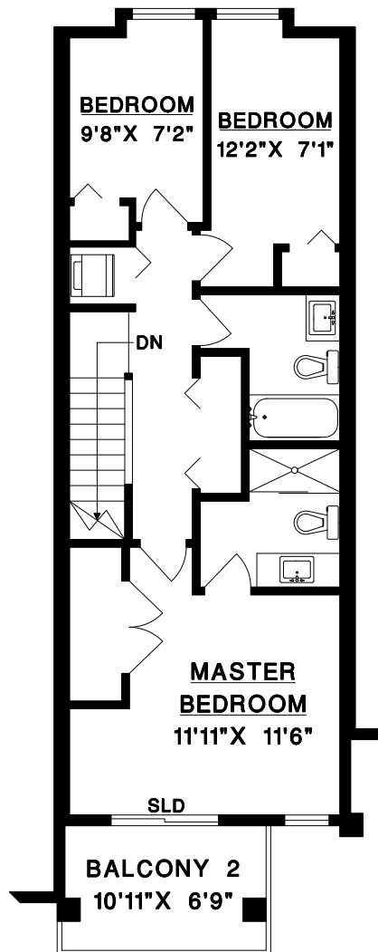
UPPER FLOOR
