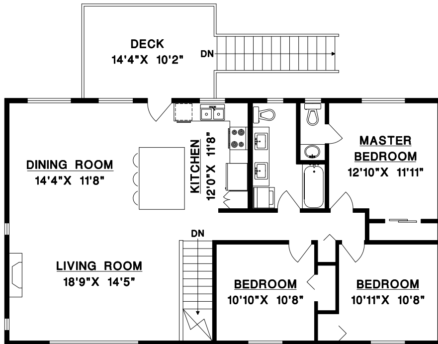
MAIN FLOOR
