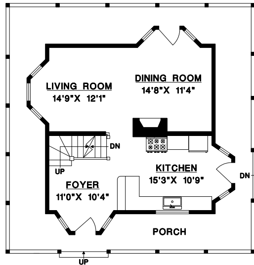
MAIN FLOOR
