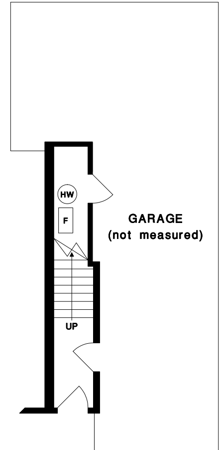
LOWER FLOOR
