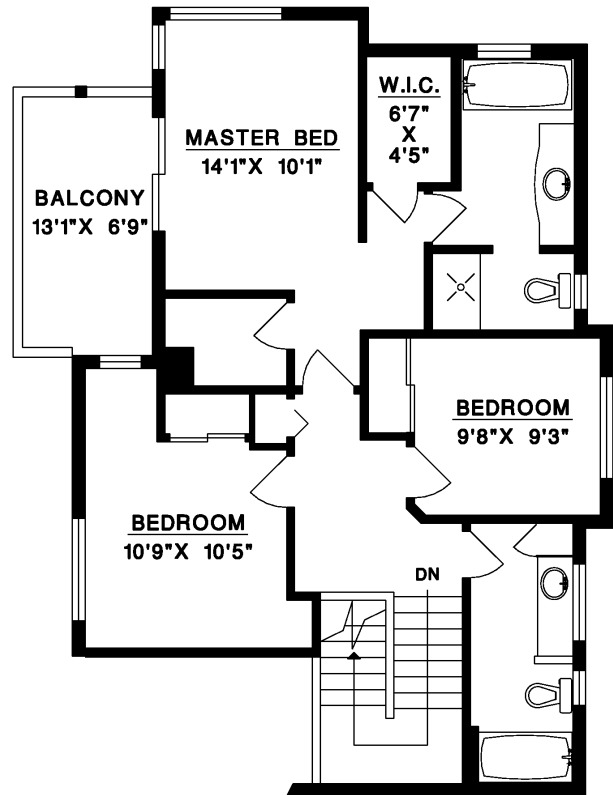
UPPER FLOOR
