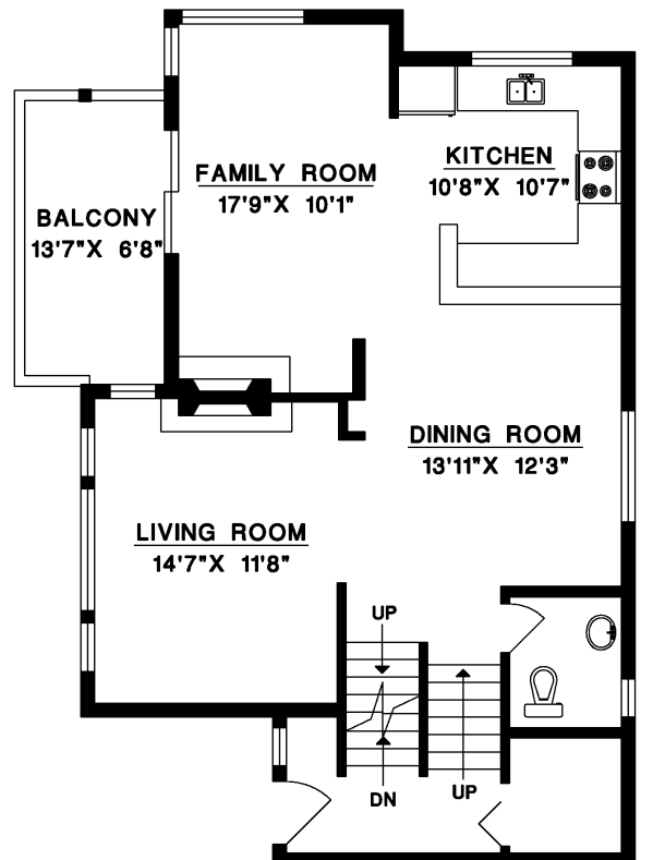
MAIN FLOOR
