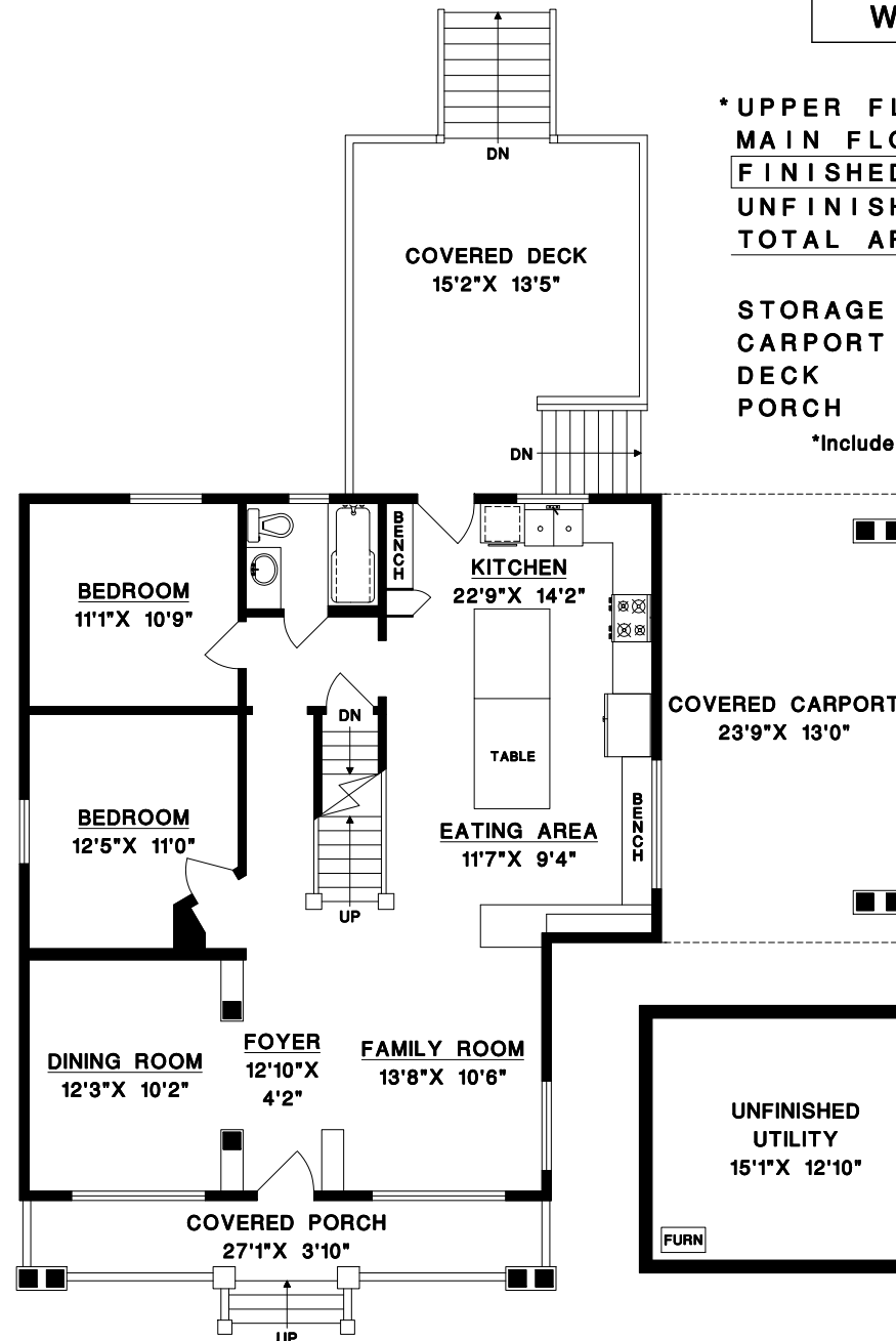
MAIN FLOOR
