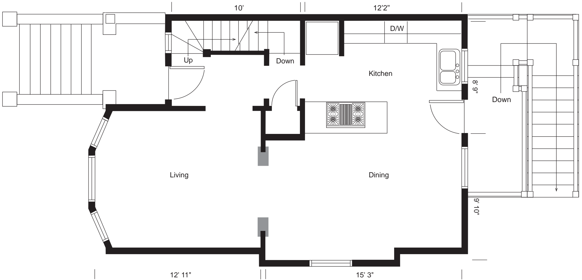
Main Floor
