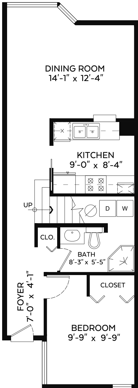
Main Floor Plan Floor Area: 608 sq.ft.
