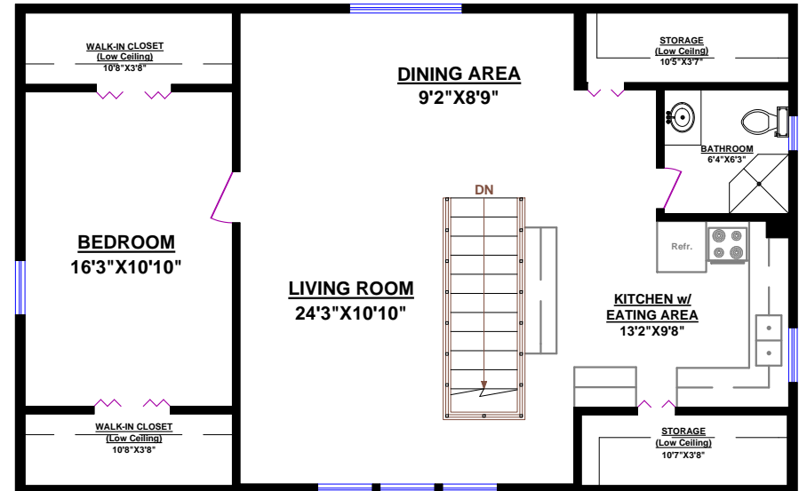
COACH HOUSE: UPPER LEVEL
