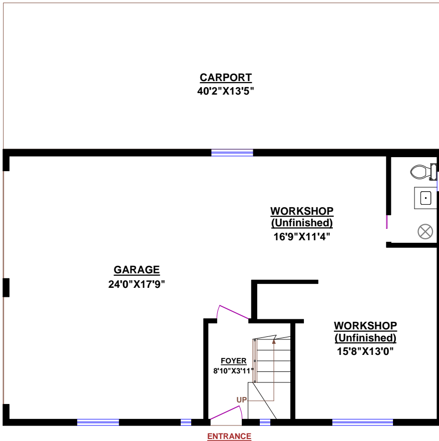
COACH HOUSE: MAIN FLOOR
