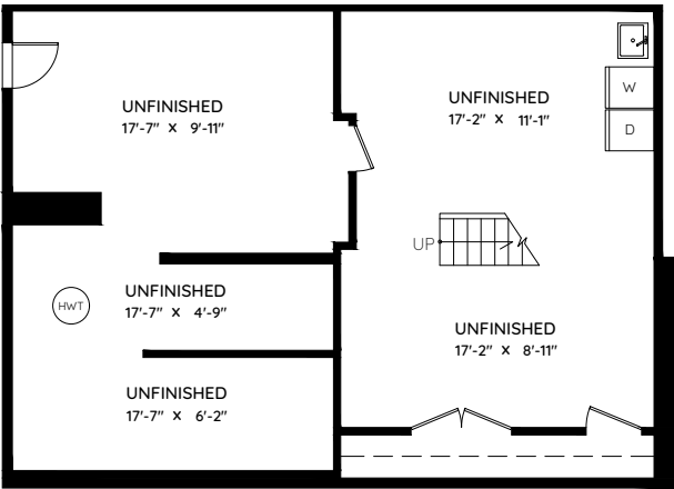
UNFINISHED LOWER FLOOR 962 SQ.FT. CH: 6'-1"
