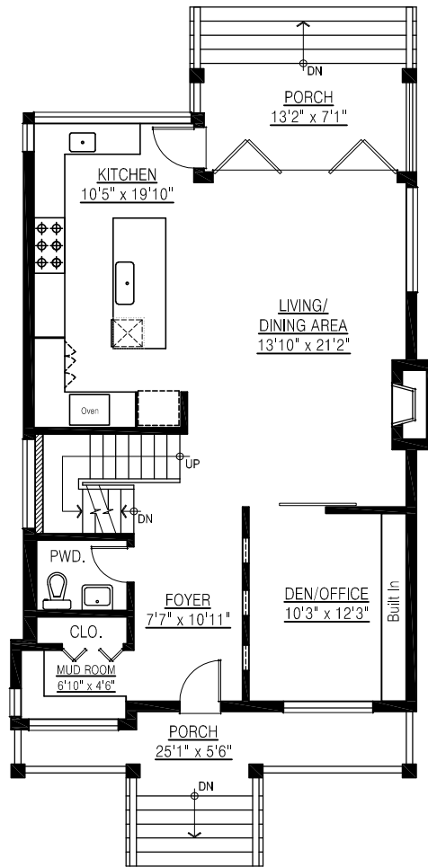
MAIN FLOOR PLAN FLOOR AREA: 958 sq.ft.
