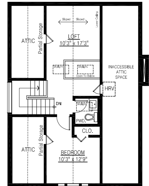
LOFT FLOOR PLAN FLOOR AREA: *373 sq.ft.
