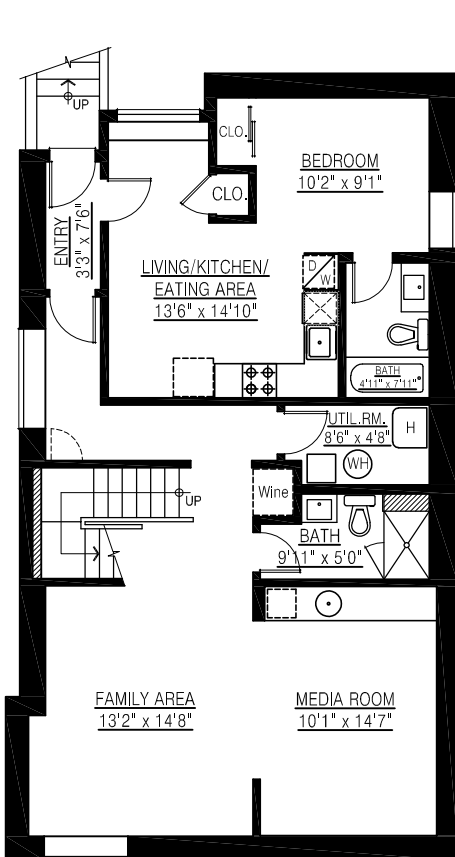
BASEMENT FLOOR PLAN FLOOR AREA: 1,136 sq.ft.
