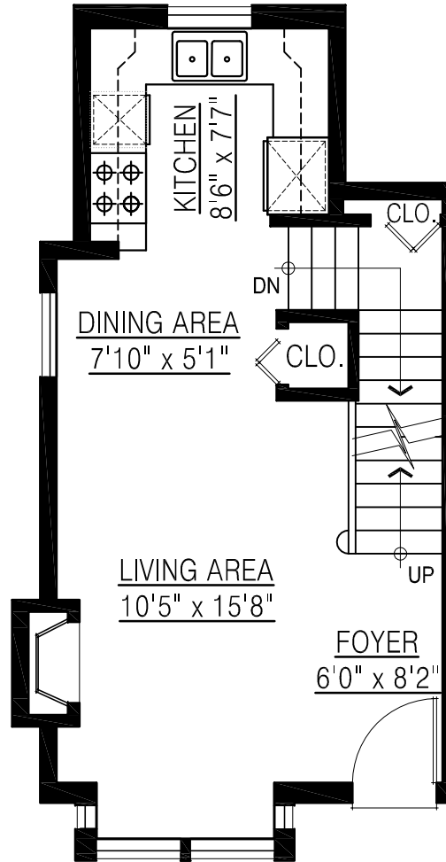
MAIN FLOOR PLAN FLOOR AREA: 402 sq. ft.
