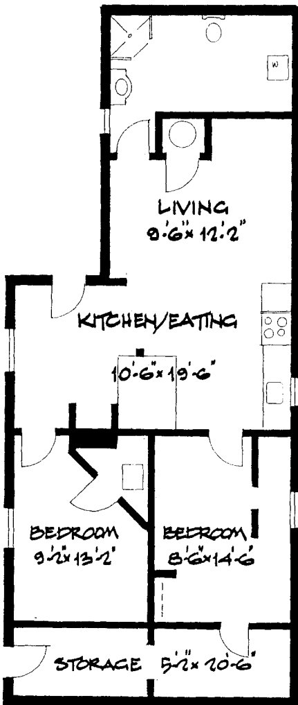
LOWER FLOOR
