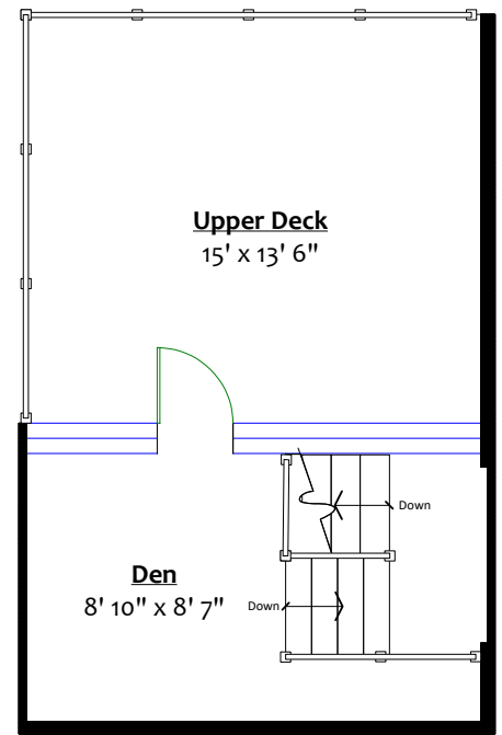
UPPER LEVEL Floor Area: 161 Sq. Ft.
